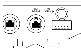
Figure 1: Front Panel LED
